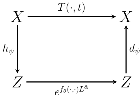
Figure 3. The commuting diagram enforced by the objective function in the latent model: T(x, t) \approx d_\psi(e^{f_\theta(x_i, \bar{x}_i)L^\alpha} h_\psi(x)) .
